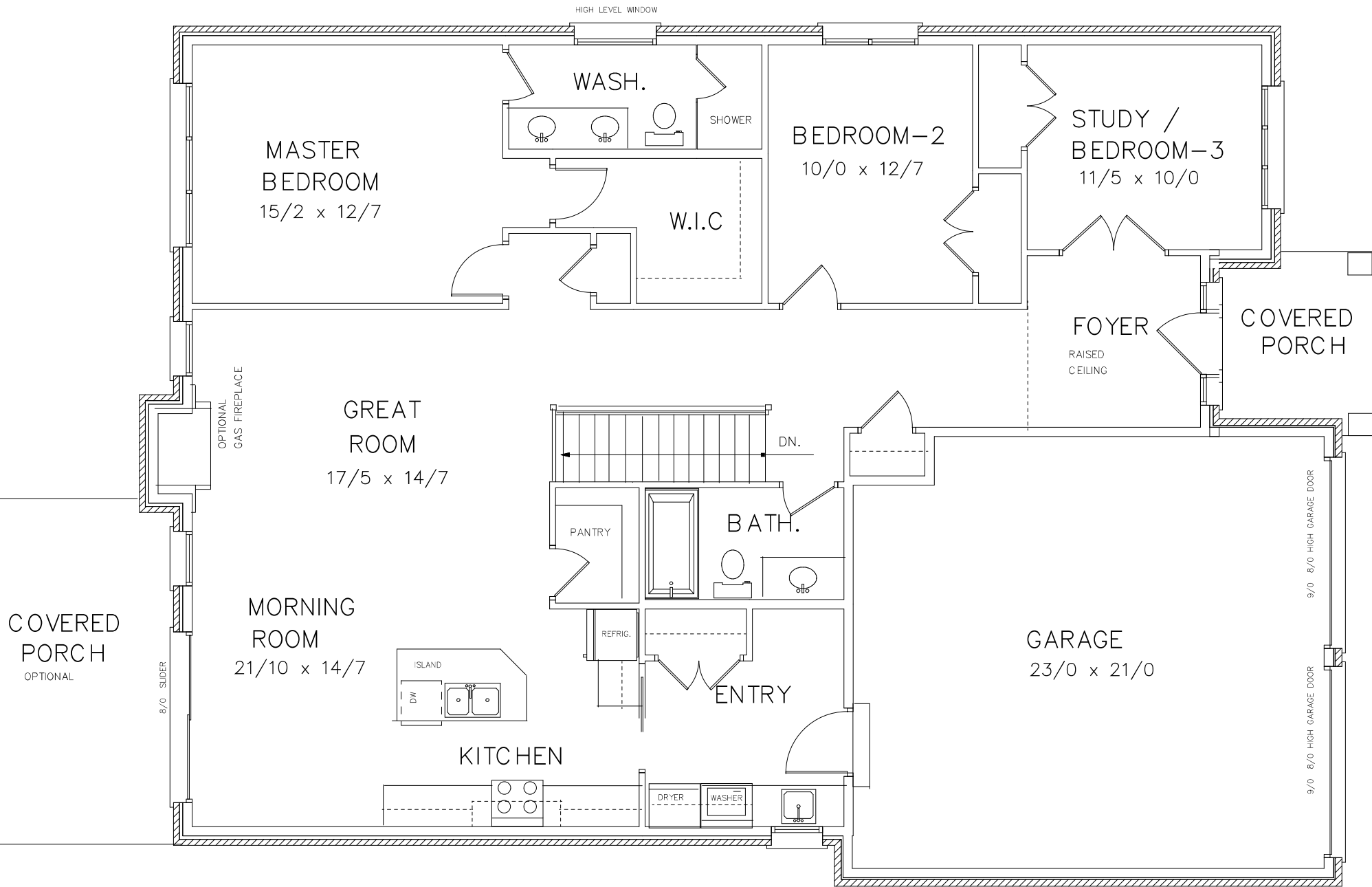
1726 SQ.FT MAIN FLOOR PLAN
