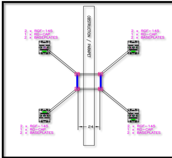
3-3 Crossover Series Stand with Platform
