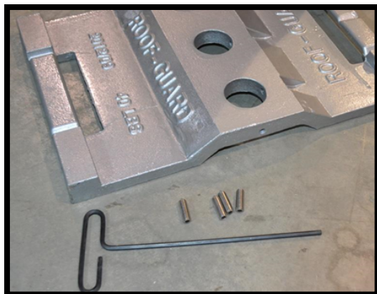
Figure 1: RoofGuard Baseplate with set screws and tool.
