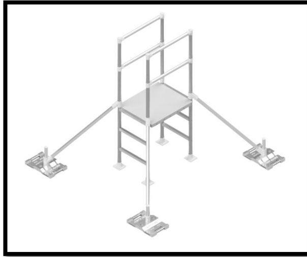
3-3 Crossover Series Stand with Platform
