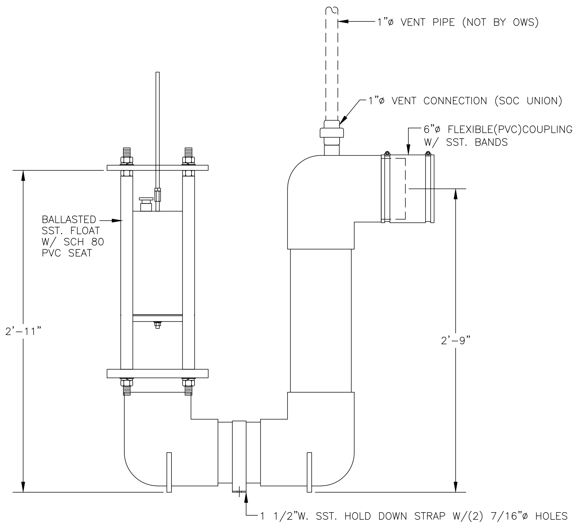
SIDE VIEW
