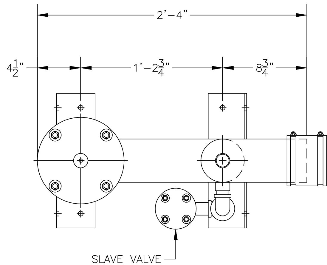
PLAN
