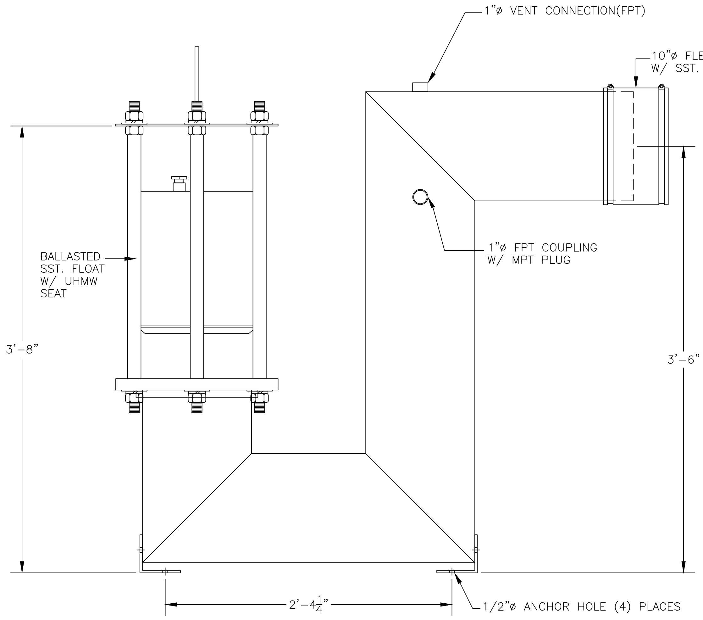
SIDE VIEW
