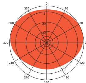
H-Plane gain 12.6 dBd 3/8 wl. spacing from tower
