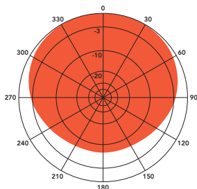
H-Plane gain 12.3 dBd 1/4 wl. spacing from tower
