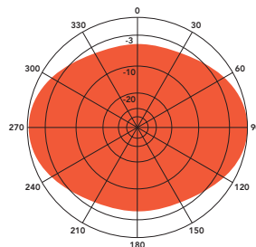
H-Plane gain 11.9 dBd 1/2 wl. spacing from tower
