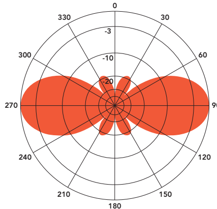
ANT790F2 - 790 MHz Vertical Plane Gain = 2.52 dBd
