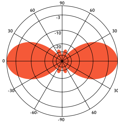
ANT425F2 - 425 MHz Vertical Plane Gain = 2.56 dBd
